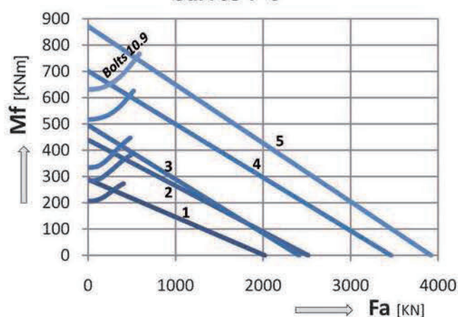
Curves 1~5
