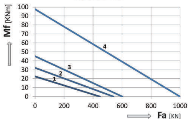
Curves 1 ~ 4
