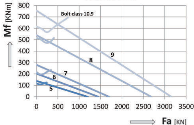
Curves 5 ~ 9
